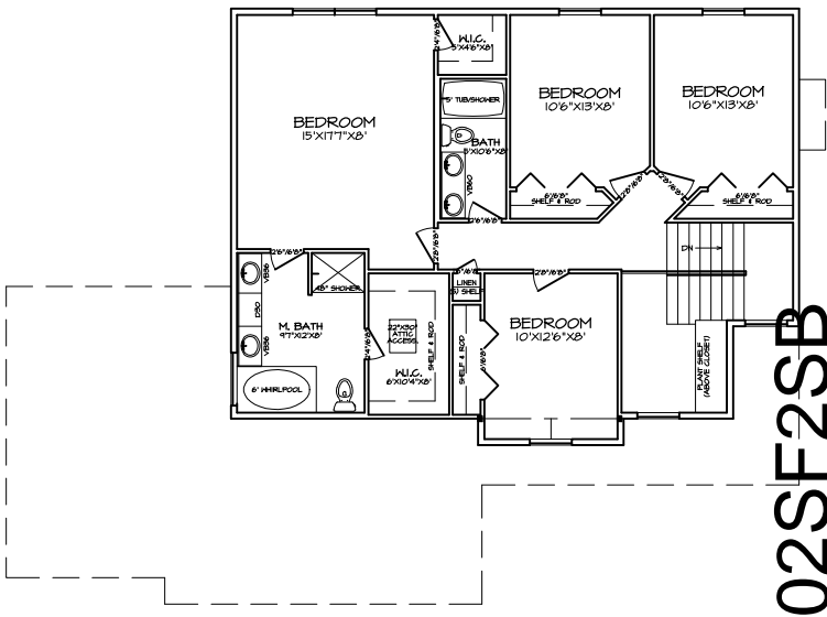
1 SECOND FLOOR PLAN A-5
