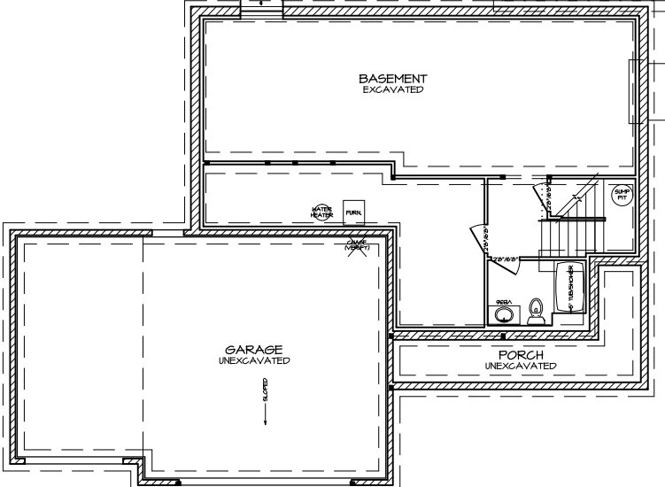
1 FOUNDATION PLAN A-3
